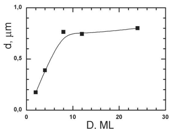
Fig. 2. The dependence of \text{Cu}_3\text{Si} nanoisland diameter on thickness of Cu deposited on Si (111).
