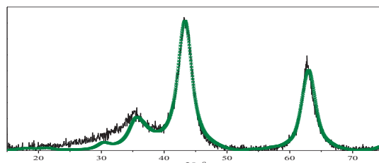
Fig.4 Simulation of the X-ray diffraction pattern for Mg-Al oxide on the base of a defective layered spinel
