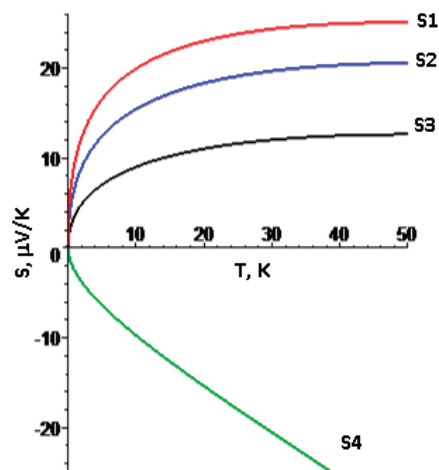
Figure 1. Temperature dependence of thermopower of the CNT (10,10), calculated for different values S(T) of short-range order: \sum\alpha_i=0.3 (S1), \sum\alpha_i=0.2 (S2), \sum\alpha_i=0.1 (S3) and \sum\alpha_i=-0.1 (S4).
