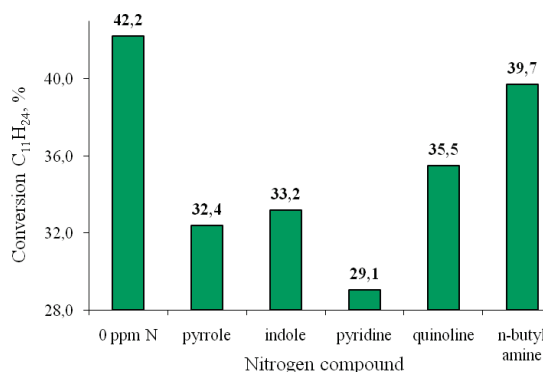
Fig. 2. The dependence of the n-undecane conversion of nitrogen compounds type (500 ppm N).
