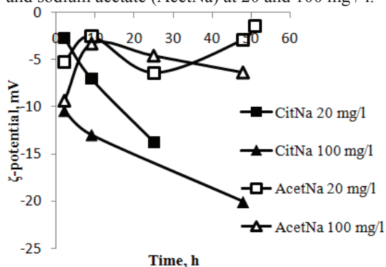
Figure 2. Change of zeta-potential of Zn particles in suspensions stabilized with sodium citrate (CitNat) and sodium acetate (AcetNa) at 20 and 100 mg / l.
