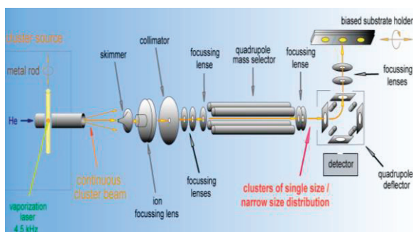
Figure 1. Schematics of the cluster deposition apparatus used for the atomic precision synthesis of model size-selected subnanometer catalysts.
