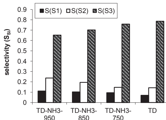
Figure 3. Differential selectivities ( S_{S1} , S_{S2} and S_{S3} ) of palladium catalysts deposited on mesoporous activated carbons in competitive Suzuki-Miyaura reaction.
