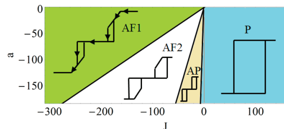
Figure 2. A magnetic phase diagram for two nanomagnets with anisotropy a and interaction strength J . There are four phases “AF1”, “AF2”, “AP” and “P” related to the shape of the magnetization hysteresis loops as shown.
