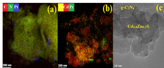
Fig. 2. Elemental mapping (a-b) and HRTEM image (c) of the photocatalyst synthesized according to Scheme 2 — 20% \text{Cd}_{0.8}\text{Zn}_{0.2}\text{S}/1\% \text{Pt}/g\text{-C}_3\text{N}_4
